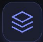
Photoshop plugin
